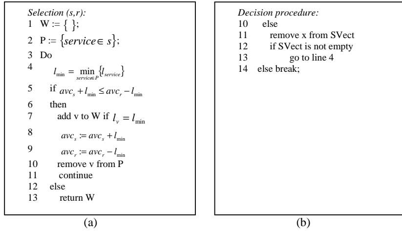
Fig. 2. The DIHomoService algorithm: (a) the Selection function, (b) the segment replacing line 10 and 11 of the Decision procedure in Fig. 1.(a).
